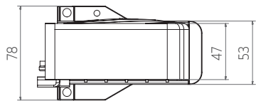
Detached controller
